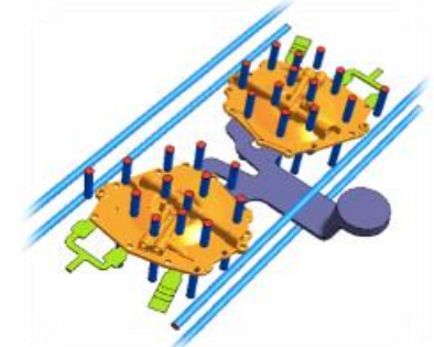
Diecasting / Gravity- Simulation
