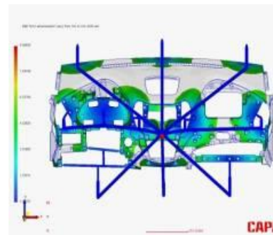
Injection plastic - Simulation
