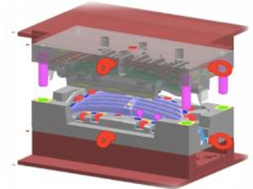
3D Injection Mold Design & Mfg.
